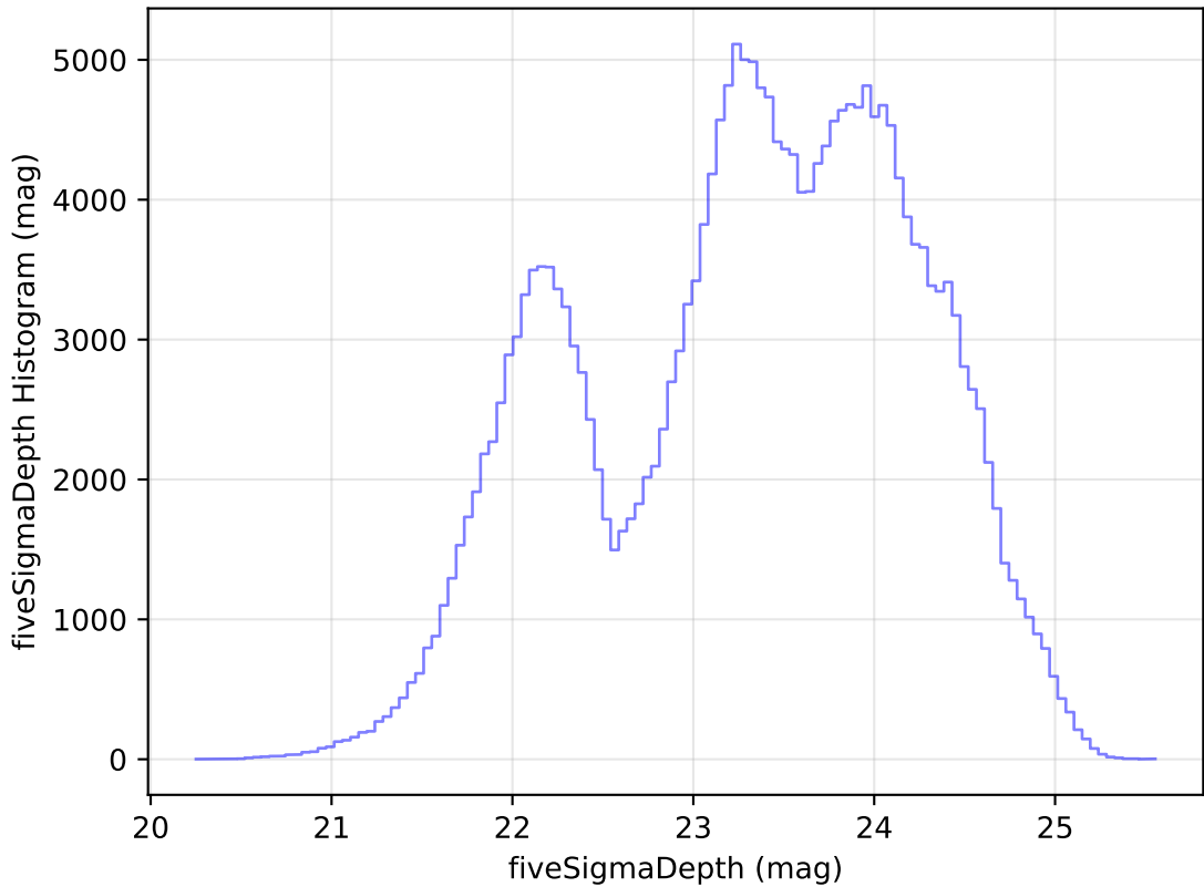
ddf_acor_sf10_lsf15_lsr20_v3.4_10yrs Yr 1 all bands: fiveSigmaDepth Histogram
