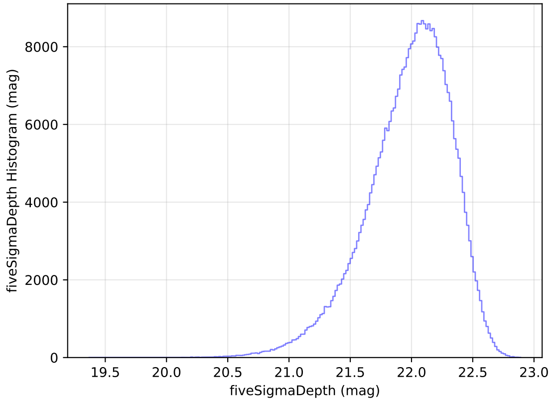
ddf_acor_sf10_lsf15_lsr20_v3.4_10yrs WFD y band: fiveSigmaDepth Histogram
