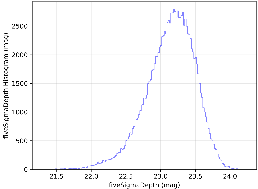
ddf_acor_sf10_lsf15_lsr20_v3.4_10yrs WFD u band: fiveSigmaDepth Histogram
