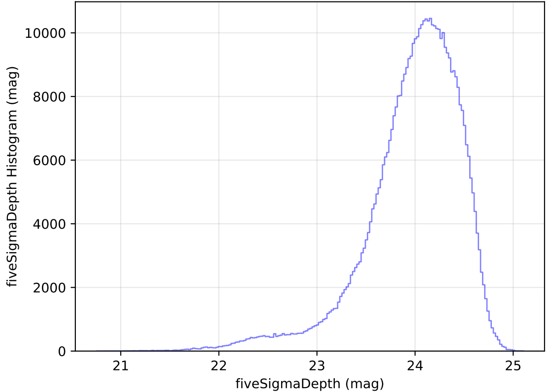
ddf_acor_sf10_lsf15_lsr20_v3.4_10yrs WFD r band: fiveSigmaDepth Histogram
