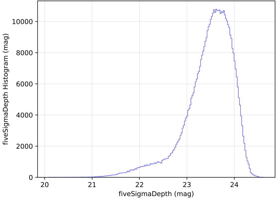
ddf_acor_sf10_lsf15_lsr20_v3.4_10yrs WFD i band: fiveSigmaDepth Histogram
