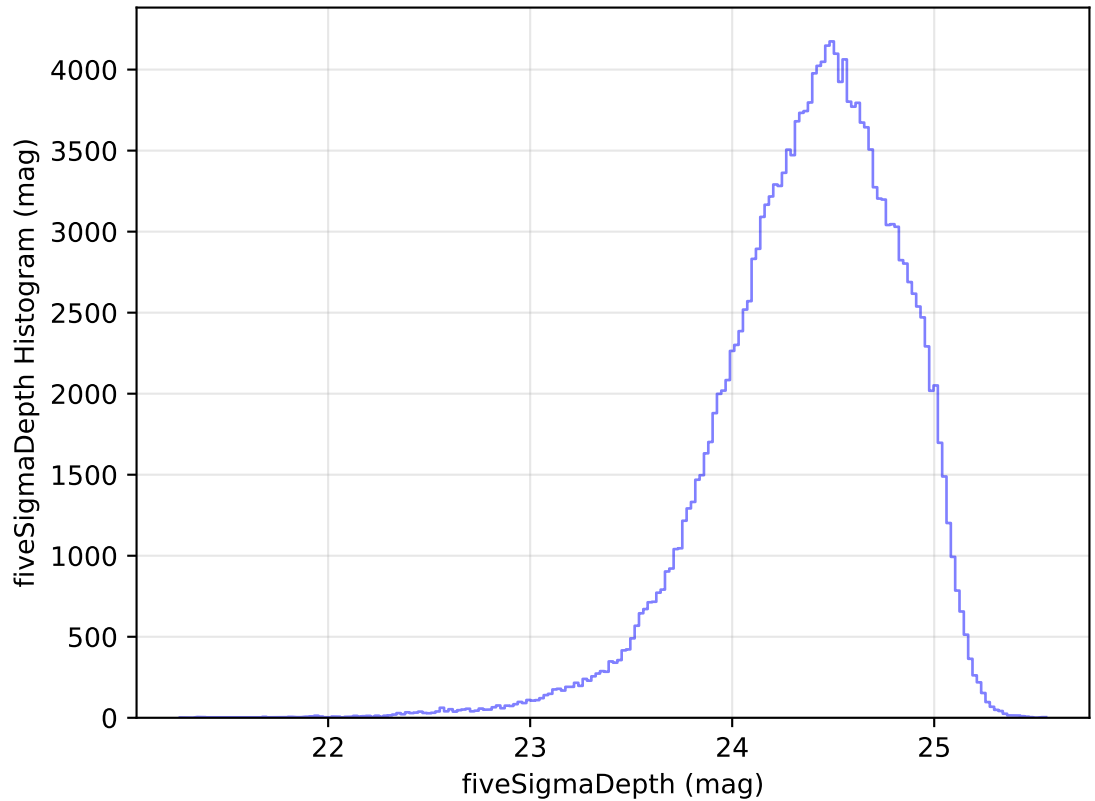
ddf_acor_sf10_lsf15_lsr20_v3.4_10yrs WFD g band: fiveSigmaDepth Histogram
