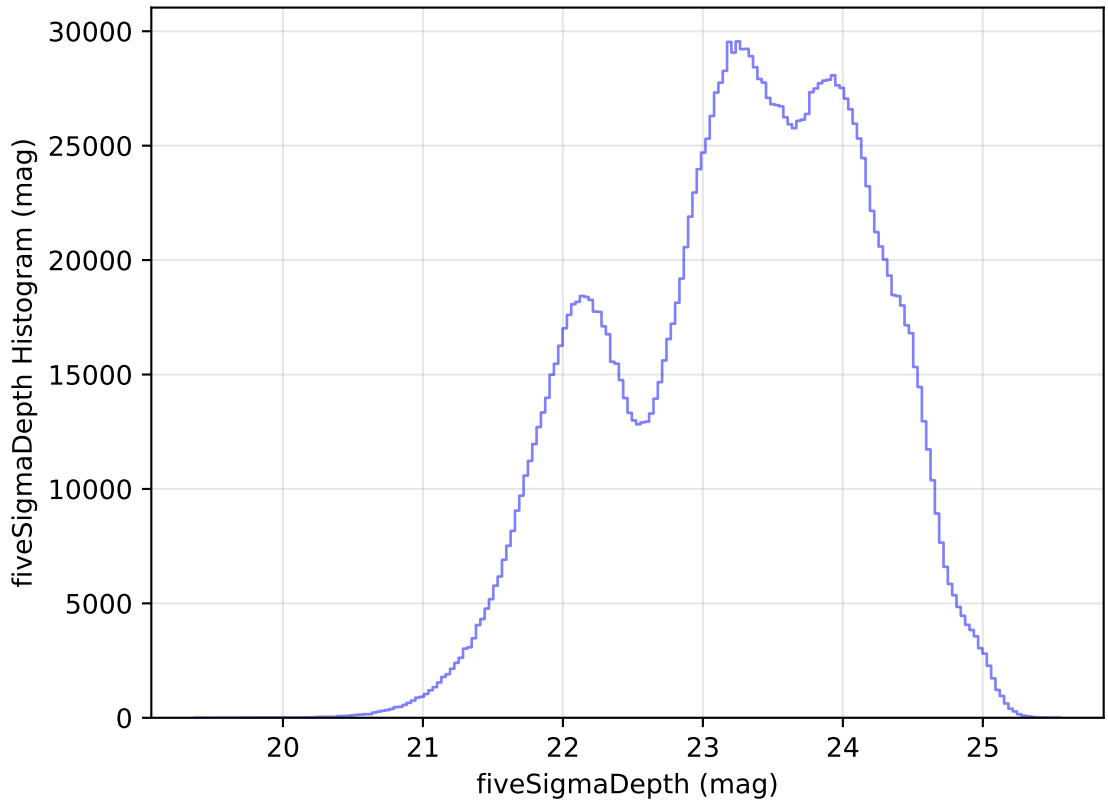
ddf_acor_sf10_lsf15_lsr20_v3.4_10yrs WFD all bands: fiveSigmaDepth Histogram
