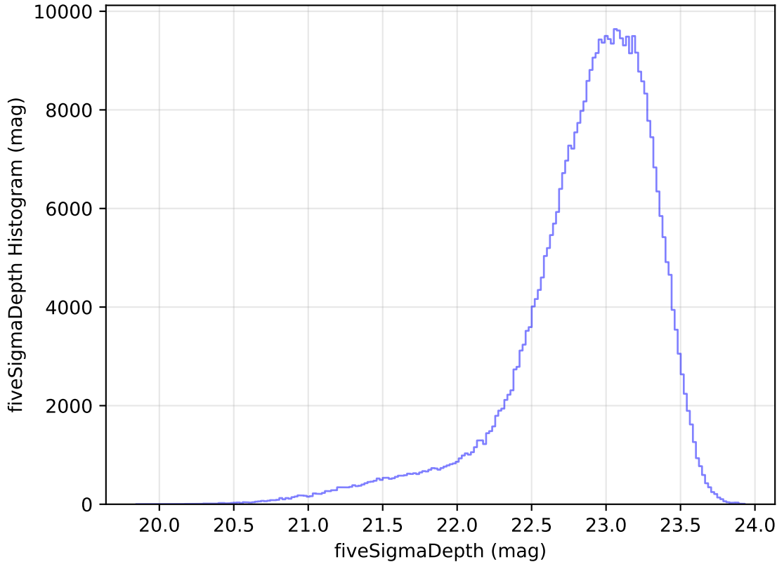
ddf_acor_sf10_ls15_lsr20_v3.4_10yrs All sky z band: fiveSigmaDepth Histogram
