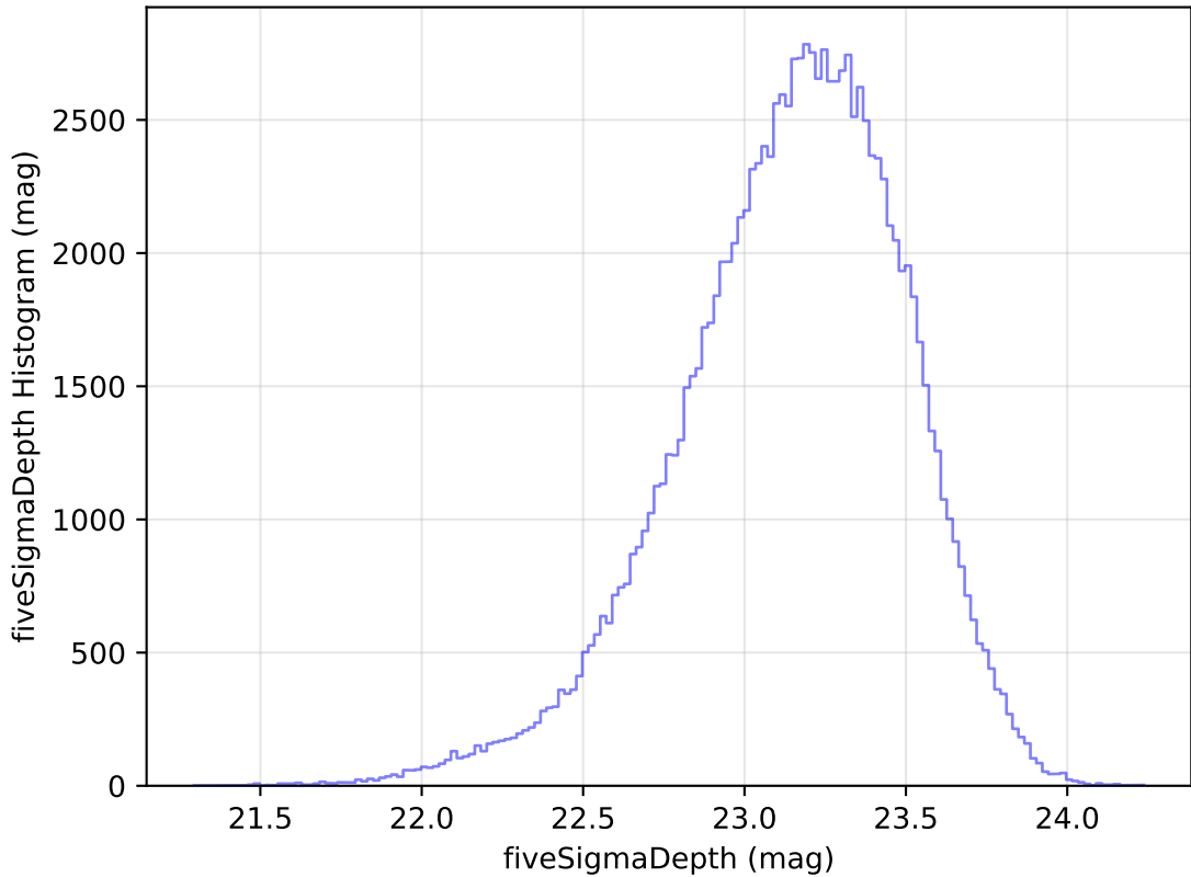
ddf_acor_sf10_lsf15_lsr20_v3.4_10yrs All sky u band: fiveSigmaDepth Histogram
