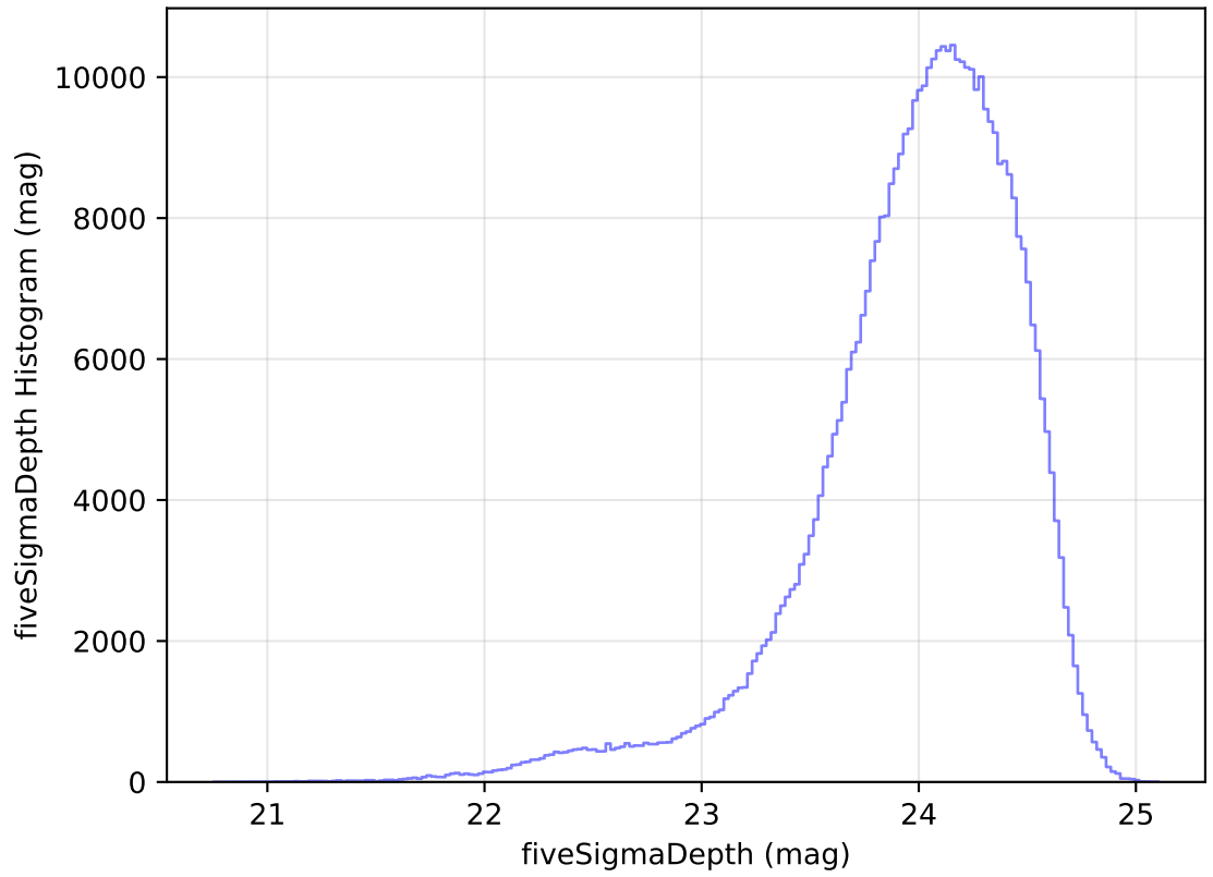
ddf_acor_sf10_ls15_lsr20_v3.4_10yrs All sky r band: fiveSigmaDepth Histogram
