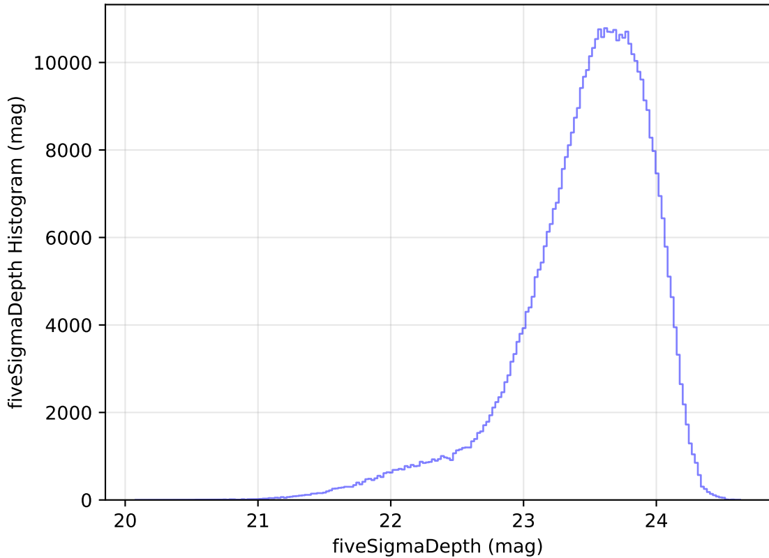
ddf_acor_sf10_lsf15_lsr20_v3.4_10yrs All sky i band: fiveSigmaDepth Histogram
