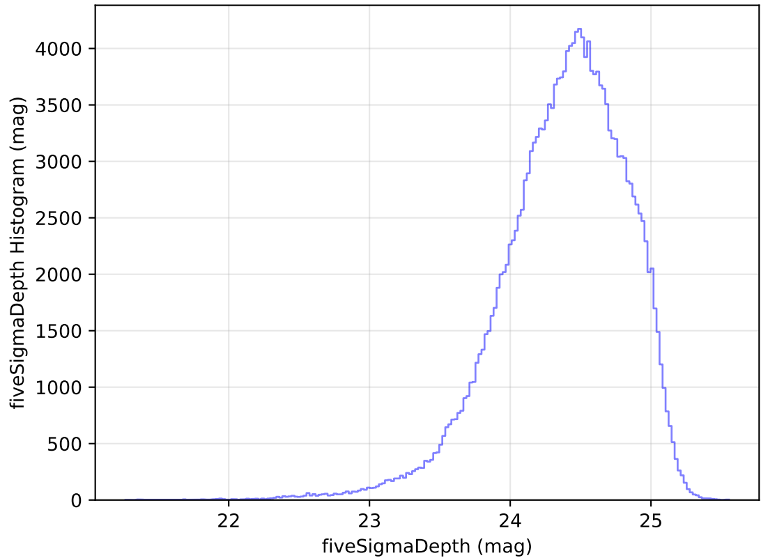
ddf_acor_sf10_lsf15_lsr20_v3.4_10yrs All sky g band: fiveSigmaDepth Histogram
