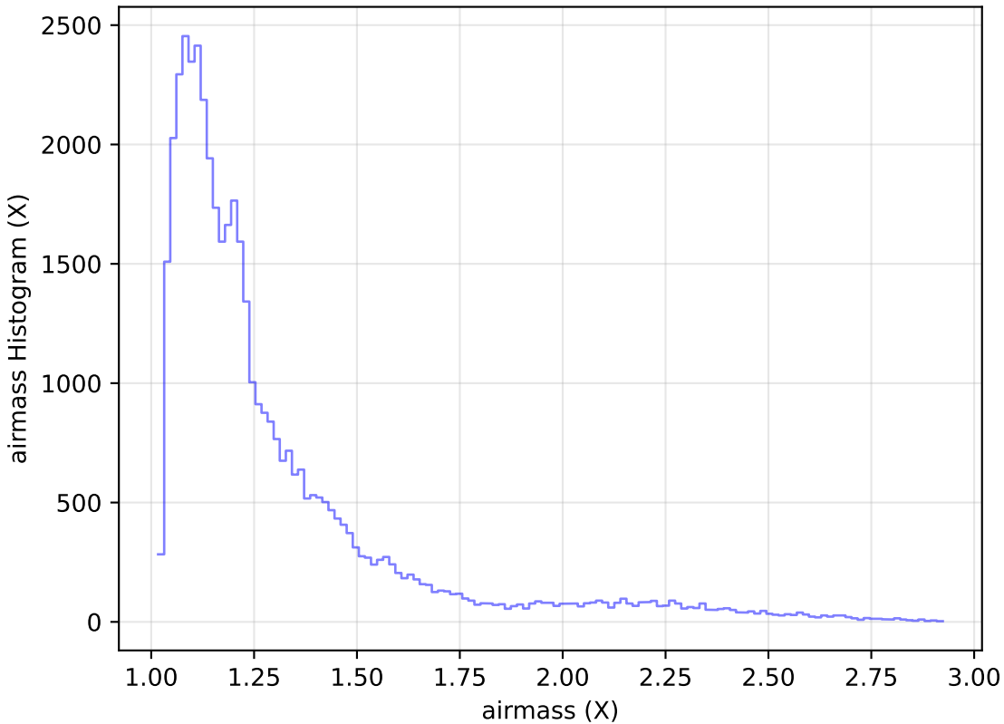
ddf_acor_sf10_lsf15_lsr20_v3.4_10yrs Yr 1 z band: airmass Histogram
