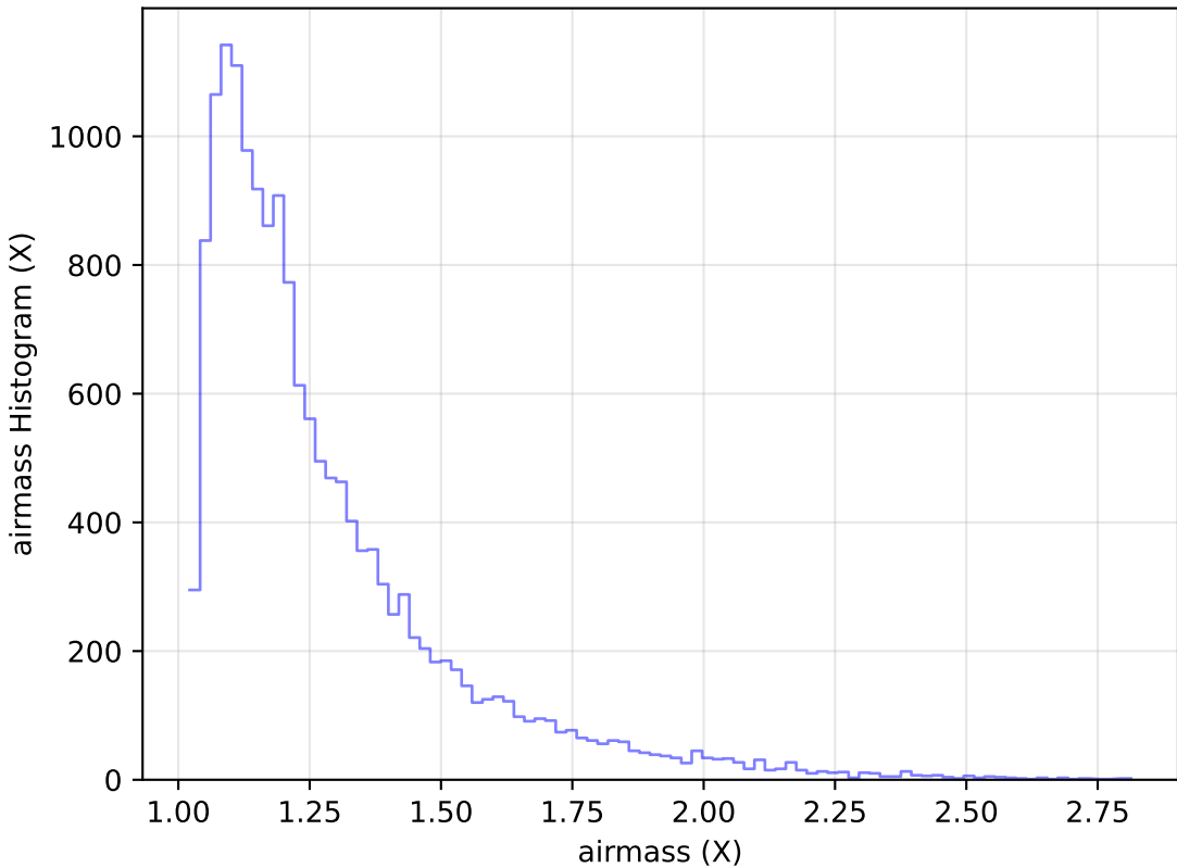
ddf_acor_sf10_ls15_lsr20_v3.4_10yrs Yr 1 u band: airmass Histogram
