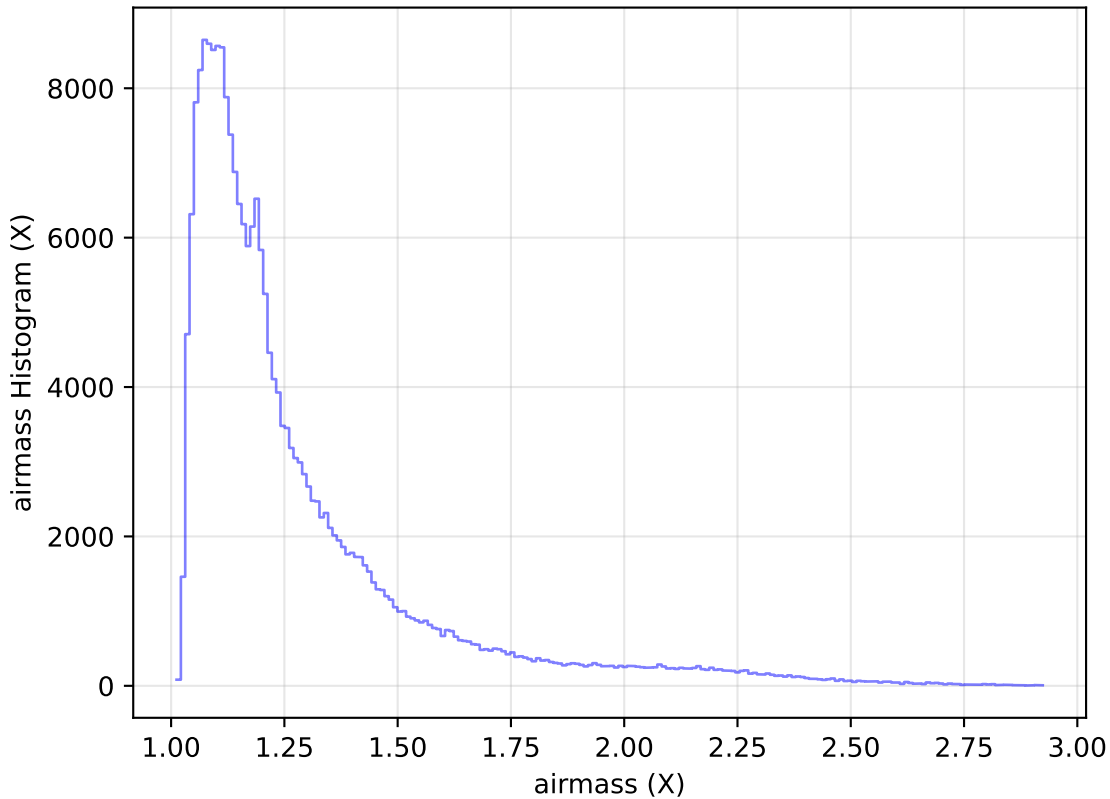
ddf_acor_sf10_lsf15_lsr20_v3.4_10yrs Yr 1 all bands: airmass Histogram
