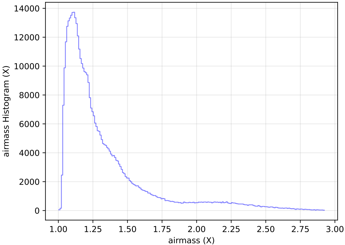
ddf_acor_sf10_lsf15_lsr20_v3.4_10yrs WFD z band: airmass Histogram
