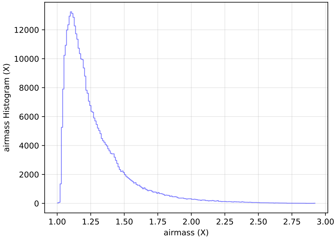
ddf_acor_sf10_lsf15_lsr20_v3.4_10yrs WFD y band: airmass Histogram
