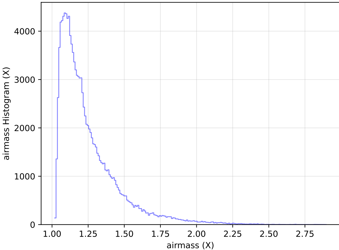
ddf_acor_sf10_lsf15_lsr20_v3.4_10yrs WFD u band: airmass Histogram
