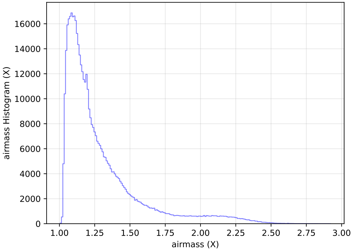
ddf_acor_sf10_lsf15_lsr20_v3.4_10yrs WFD r band: airmass Histogram
