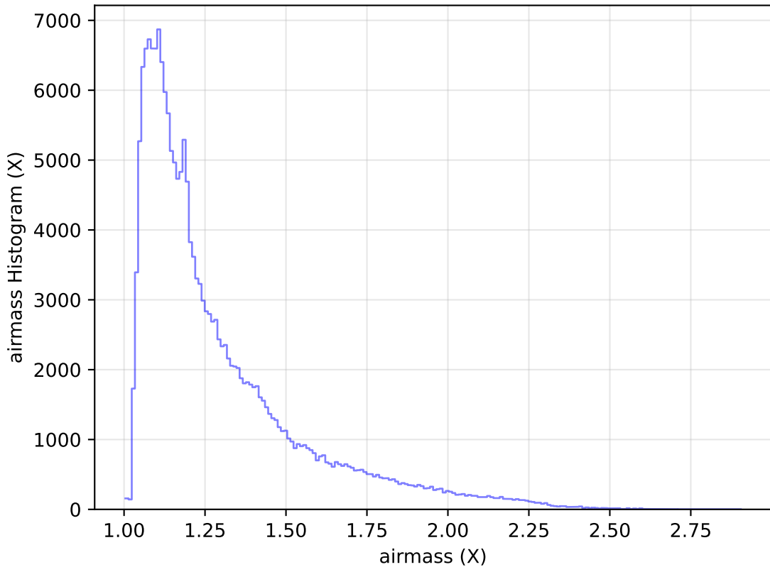
ddf_acor_sf10_ls15_lsr20_v3.4_10yrs WFD g band: airmass Histogram
