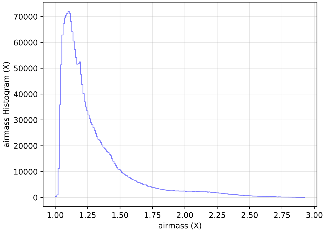
ddf_acor_sf10_lsf15_lsr20_v3.4_10yrs WFD all bands: airmass Histogram
