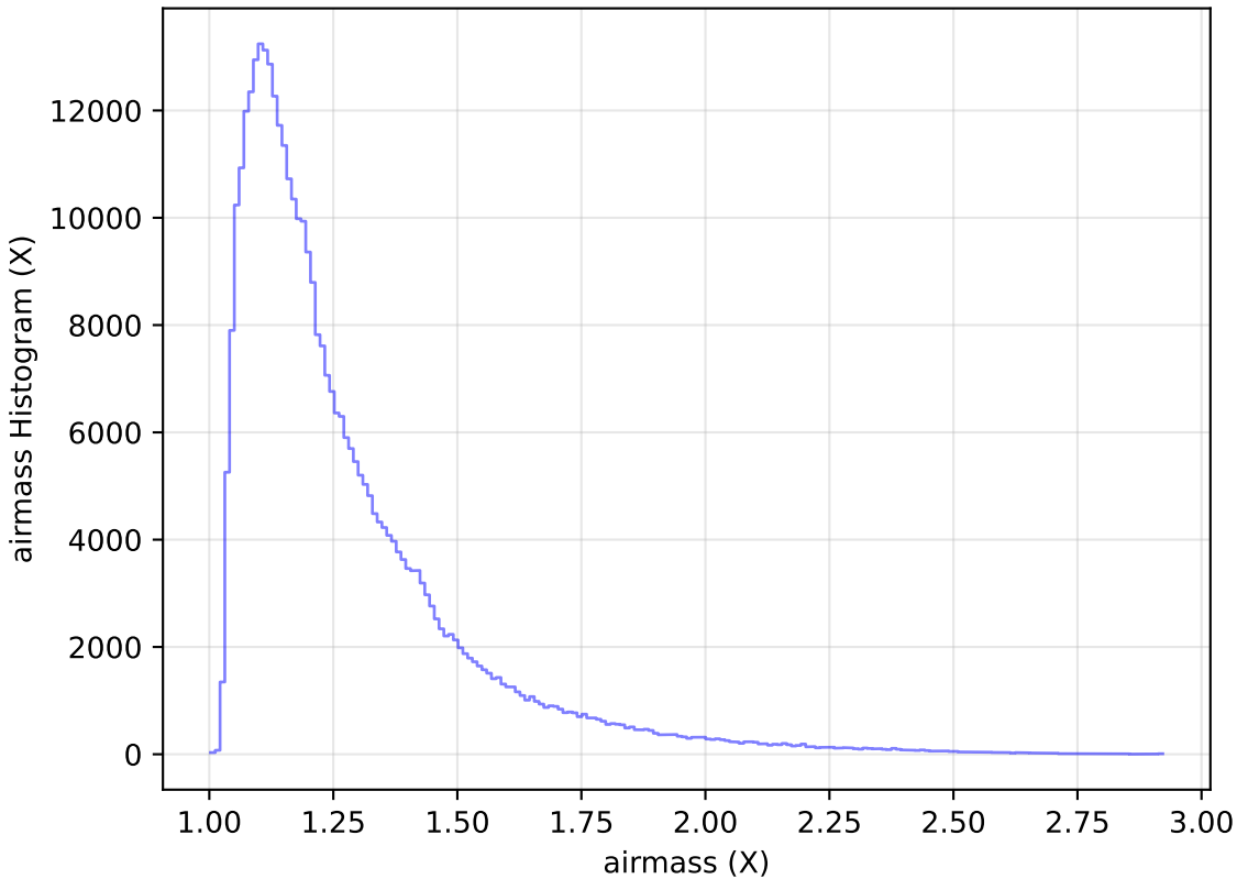
ddf_acor_sf10_ls15_lsr20_v3.4_10yrs All sky y band: airmass Histogram
