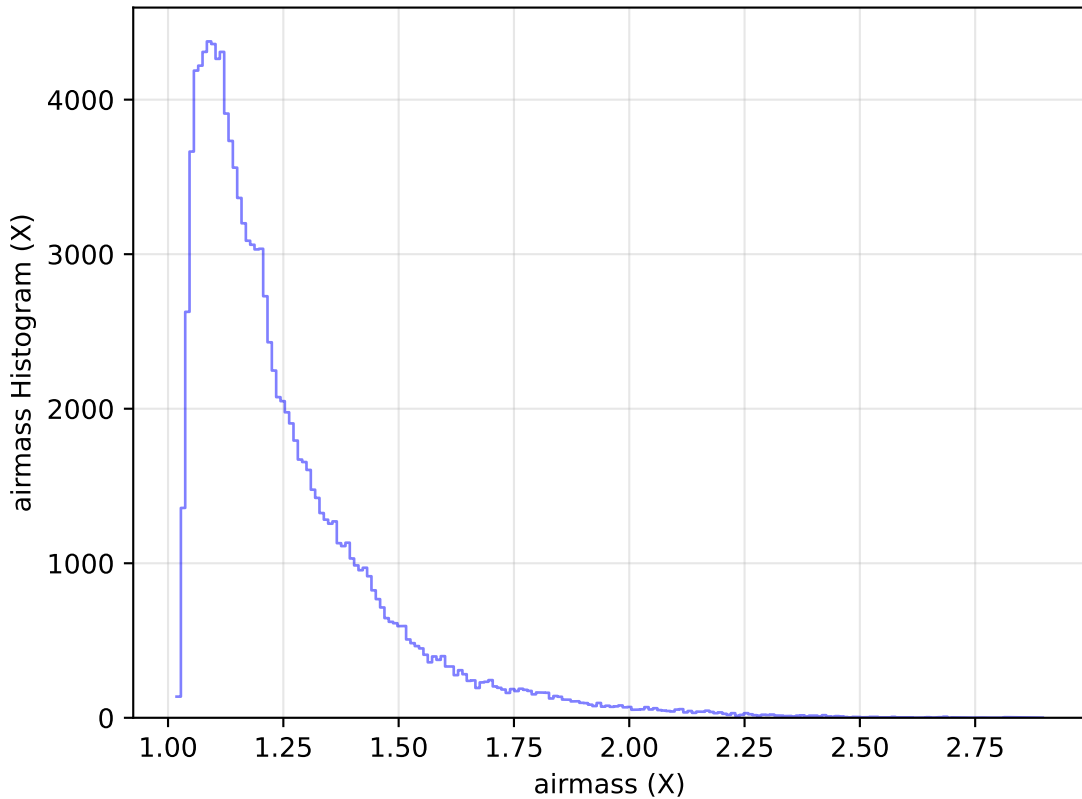
ddf_acor_sf10_lsf15_lsr20_v3.4_10yrs All sky u band: airmass Histogram
