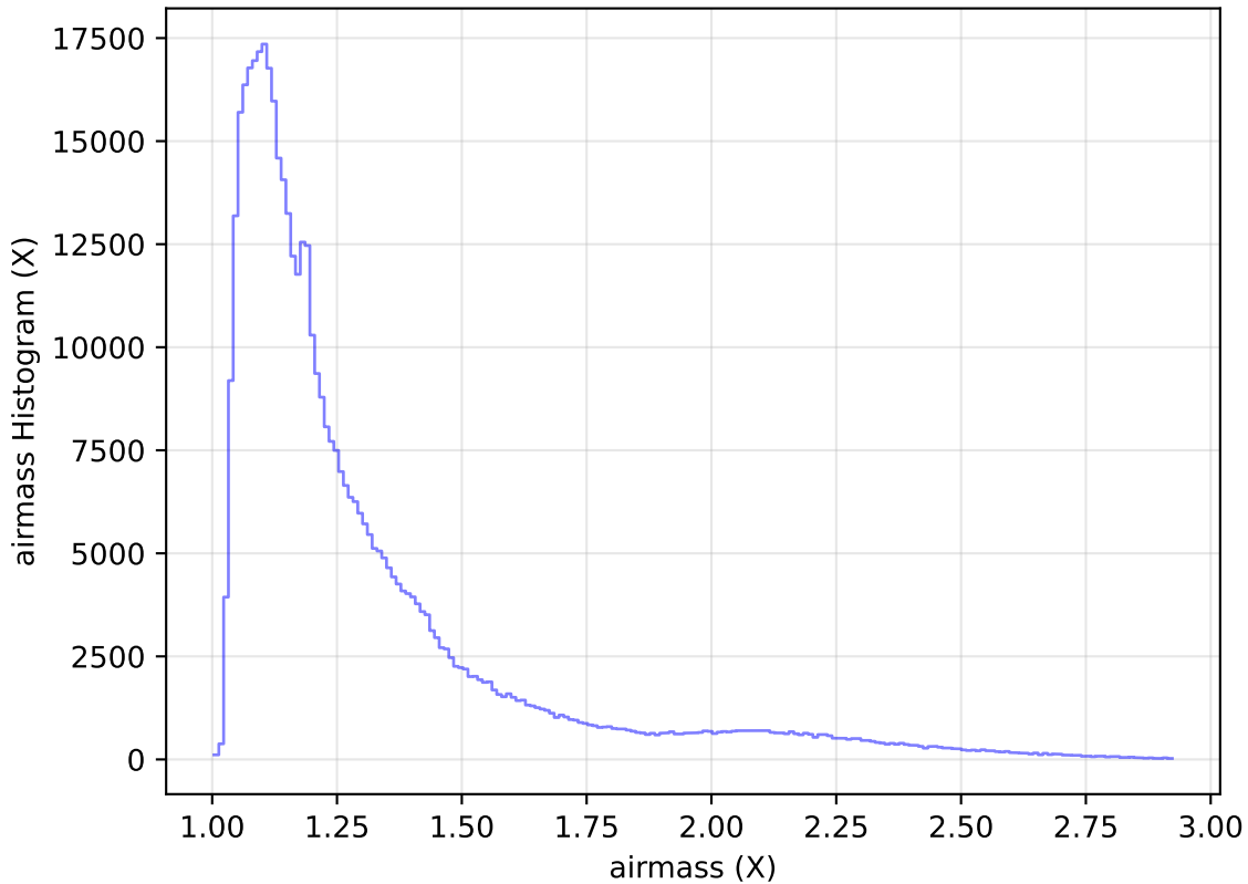
ddf_acor_sf10_lsf15_lsr20_v3.4_10yrs All sky i band: airmass Histogram
