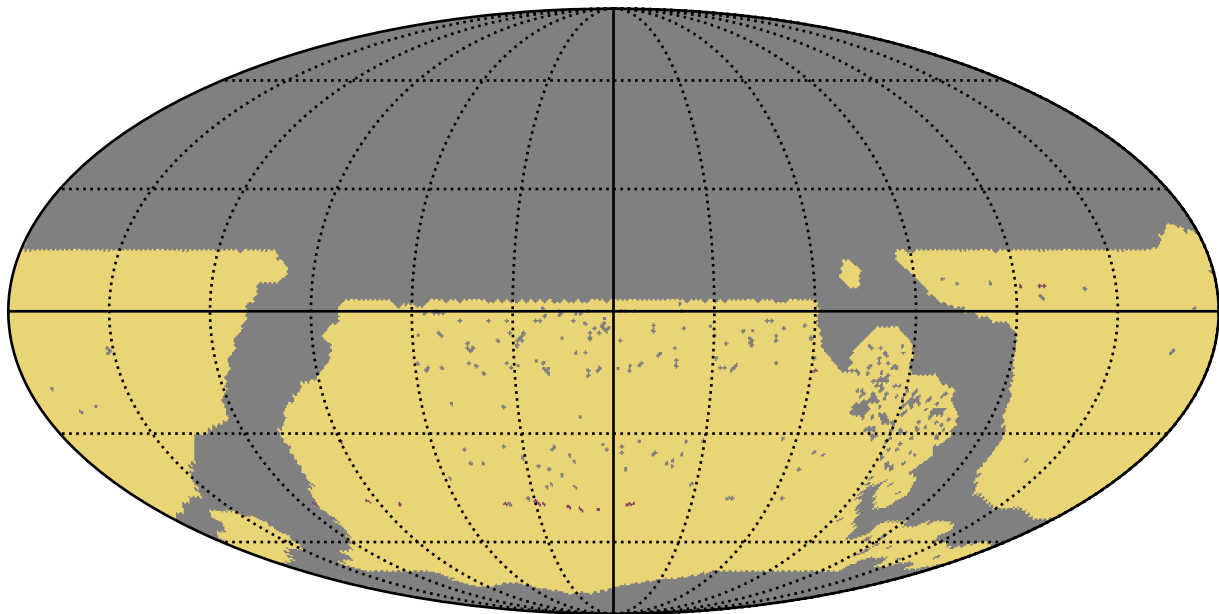
ddf_acor_sf10_lsf15_lsr20_v3.4_10yrs WFD: RapidRevisits
