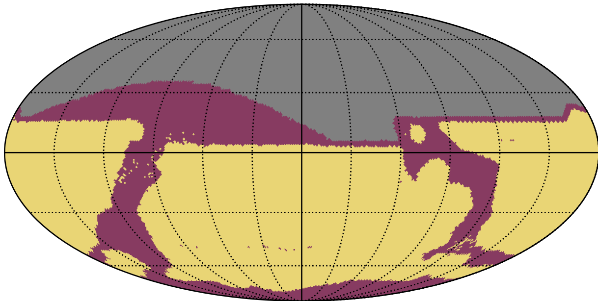
ddf_acor_sf10_lsf15_lsr20_v3.4_10yrs All sky: RapidRevisits
