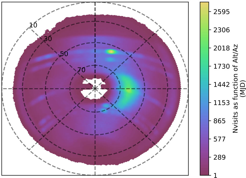
ddf_acor_sf10_lsf15_lsr20_v3.4_10yrs z band: Nvisits as function of Alt/Az
