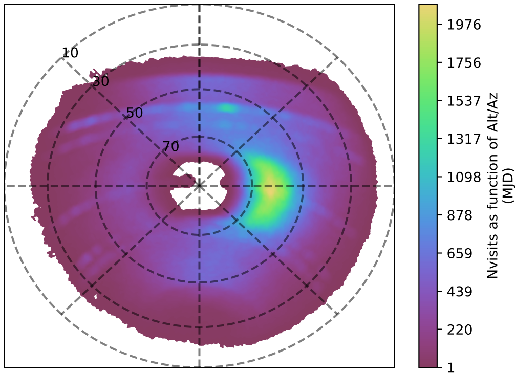
ddf_acor_sf10_lsf15_lsr20_v3.4_10yrs y band: Nvisits as function of Alt/Az
