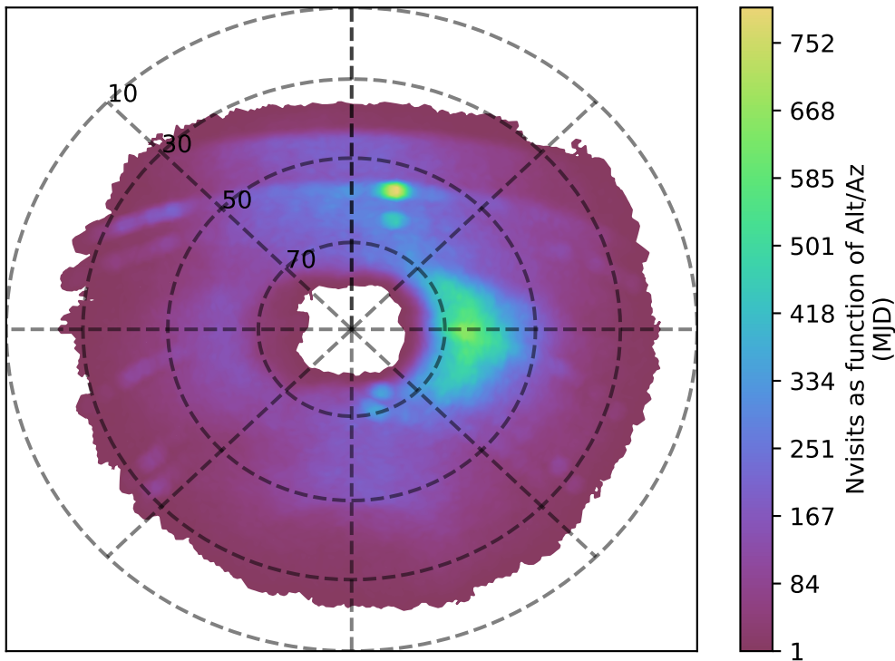
ddf_acor_sf10_ls15_lsr20_v3.4_10yrs u band: Nvisits as function of Alt/Az
