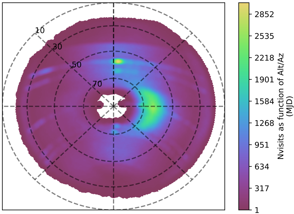
ddf_acor_sf10_lsf15_lsr20_v3.4_10yrs i band: Nvisits as function of Alt/Az
