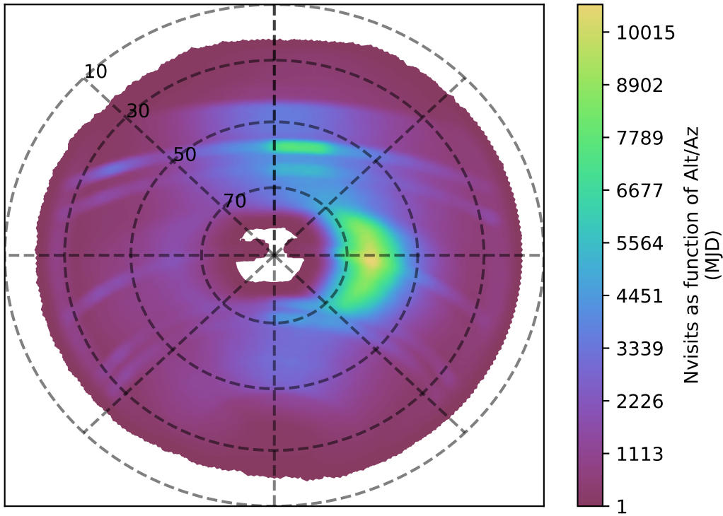
ddf_acor_sf10_ls15_lsr20_v3.4_10yrs all bands: Nvisits as function of Alt/Az
