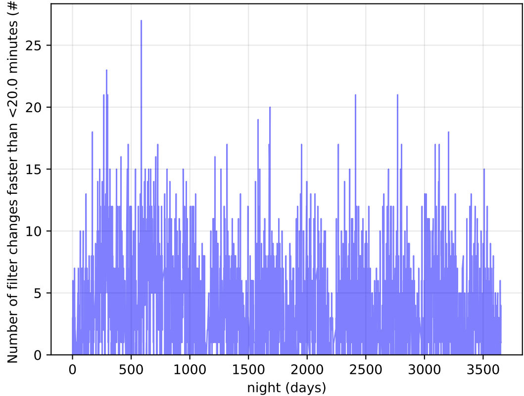
ddf_acor_sf10_Isf15_Isr20_v3.4_10yrs Per Night: Number of filter changes faster than <20.0 minutes
