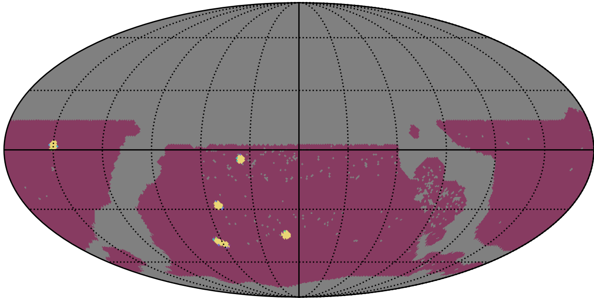
ddf_acor_sf10_lsf15_lsr20_v3.4_10yrs WFD: NumberOfQuickRevisits
