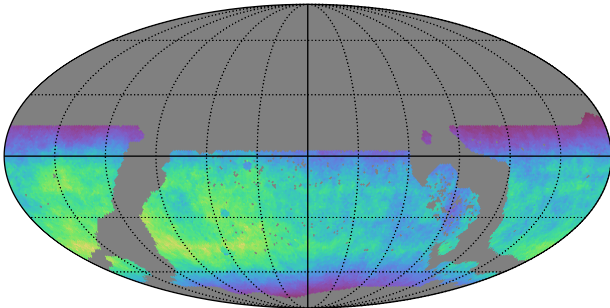
ddf_acor_sf10_lsf15_lsr20_v3.4_10yrs WFD y band: Normalized Teff
