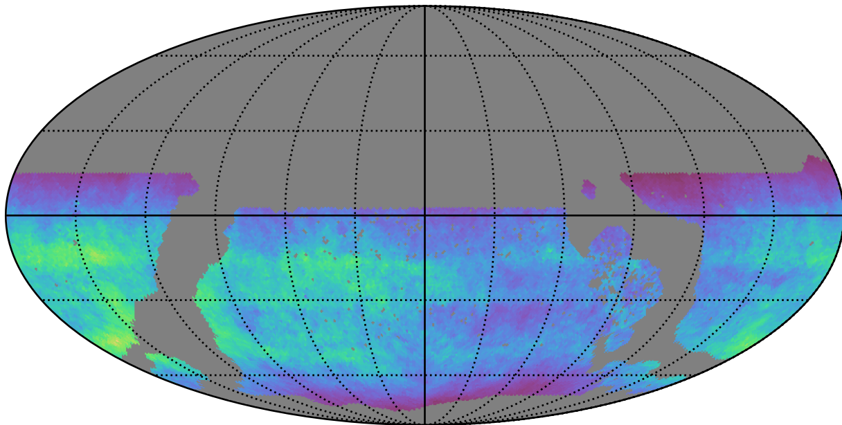
ddf_acor_sf10_lsf15_lsr20_v3.4_10yrs WFD u band: Normalized Teff
