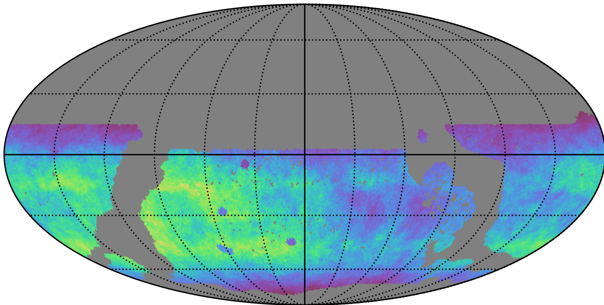
ddf_acor_sf10_lsf15_lsr20_v3.4_10yrs WFD g band: Normalized Teff
