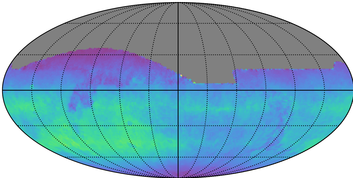
ddf_acor_sf10_lsf15_lsr20_v3.4_10yrs All sky z band: Normalized Teff
