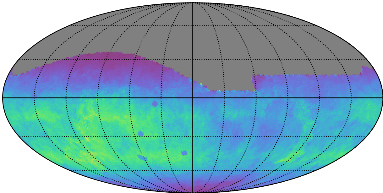
ddf_acor_sf10_lsf15_lsr20_v3.4_10yrs All sky g band: Normalized Teff
