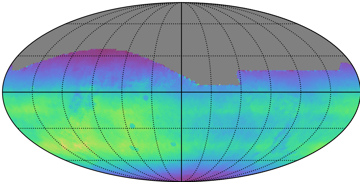
ddf_acor_sf10_lsf15_lsr20_v3.4_10yrs All sky all bands: Normalized Teff
