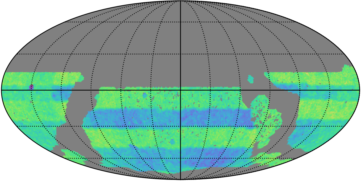
ddf_acor_sf10_lsf15_lsr20_v3.4_10yrs WFD: Normalized Proper Motion Uncert @ 20.5
