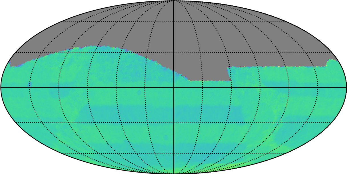
ddf_acor_sf10_lsf15_lsr20_v3.4_10yrs All sky: Normalized Proper Motion Uncert @ 20.5
