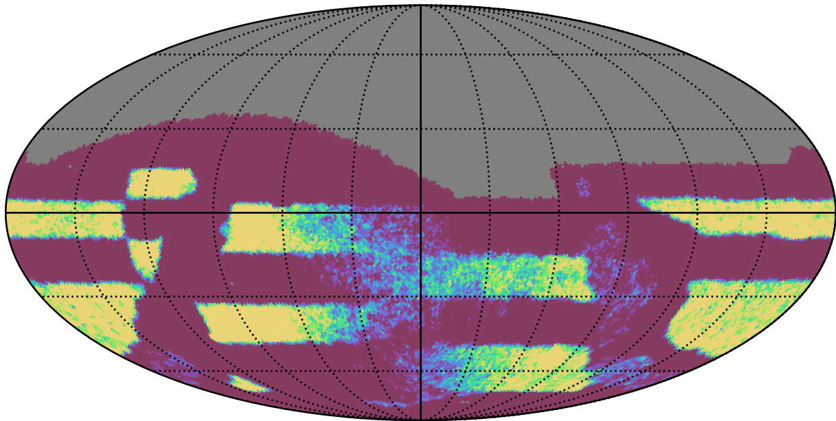
ddf_acor_sf10_lsf15_lsr20_v3.4_10yrs Yr 3-4 all bands: NVisits
