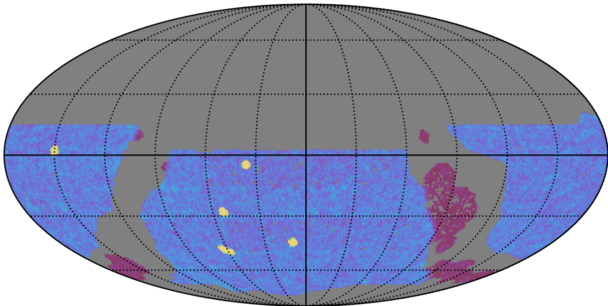
ddf_acor_sf10_lsf15_lsr20_v3.4_10yrs WFD y band: NVisits
