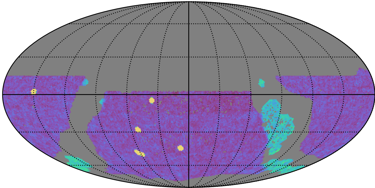
ddf_acor_sf10_lsf15_lsr20_v3.4_10yrs WFD g band: NVisits
