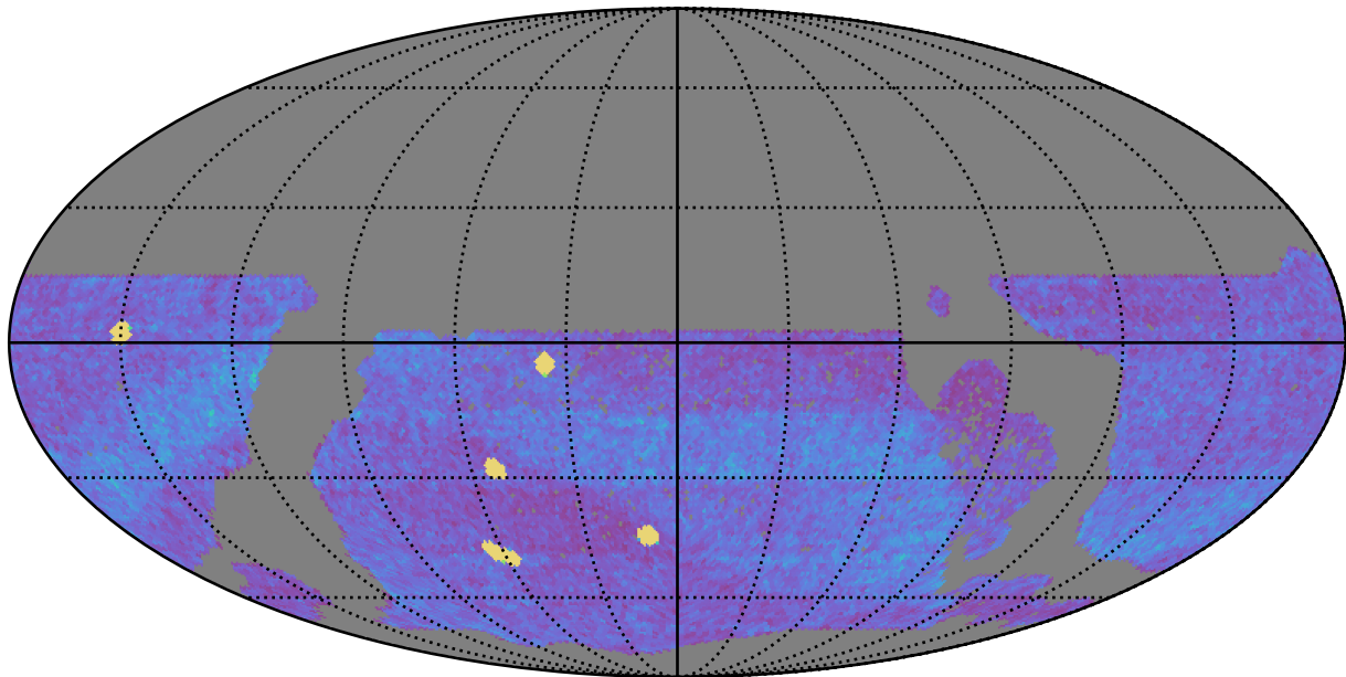
ddf_acor_sf10_lsf15_lsr20_v3.4_10yrs WFD all bands: NVisits
