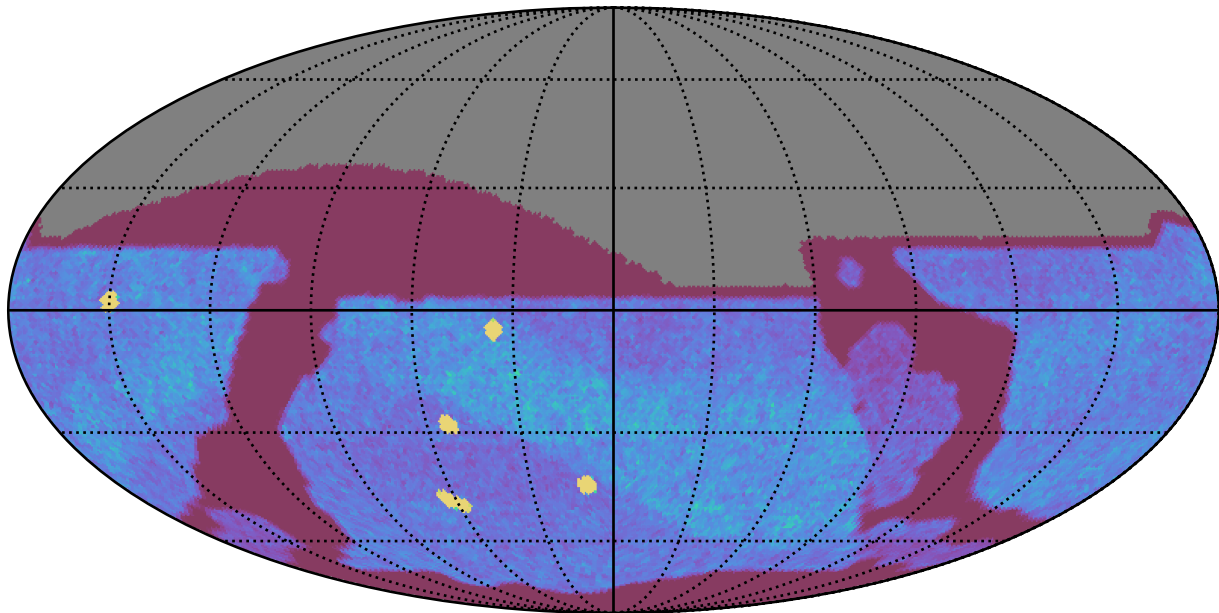
ddf_acor_sf10_lsf15_lsr20_v3.4_10yrs All sky z band: NVisits
