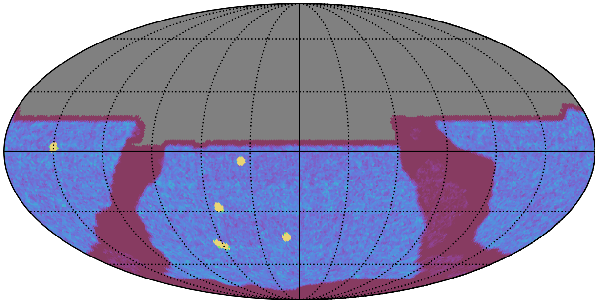
ddf_acor_sf10_lsf15_lsr20_v3.4_10yrs All sky y band: NVisits
