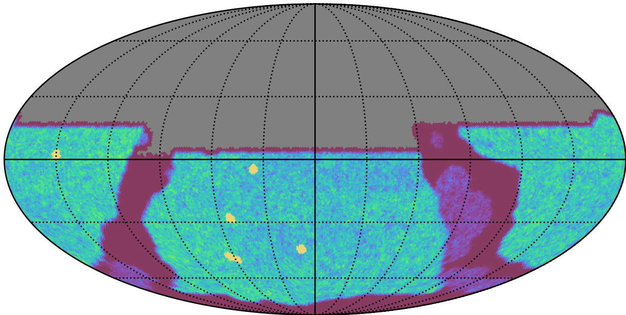
ddf_acor_sf10_lsf15_lsr20_v3.4_10yrs All sky u band: NVisits
