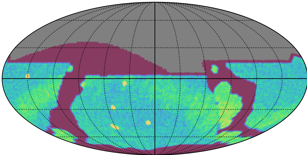
ddf_acor_sf10_lsf15_lsr20_v3.4_10yrs All sky r band: NVisits
