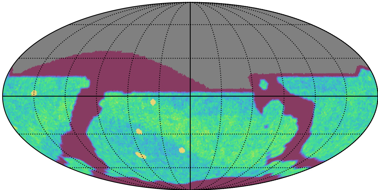
ddf_acor_sf10_lsf15_lsr20_v3.4_10yrs All sky i band: NVisits
